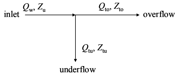
Figure 5: Thickener model assumption
